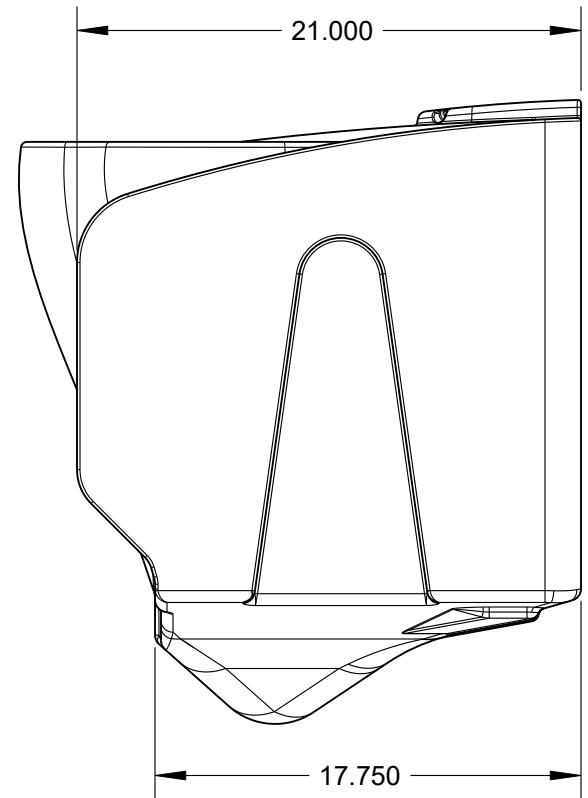
PJN3-0008 WASTE TANK PART WEIGHT: 27 LBS.
